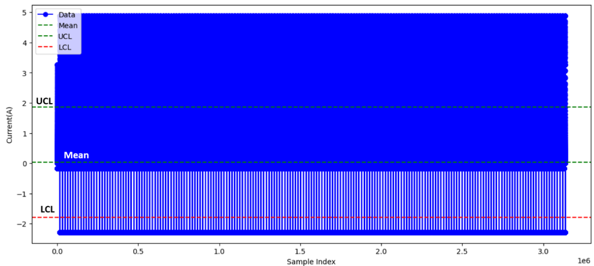
Figure 6. The control chart for current for all samples
