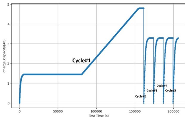
Figure 3. Change in charge capacity over test time across multiple cycles
