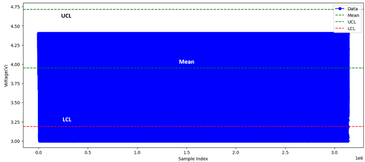
Figure 5. The control chart for voltage for all samples
