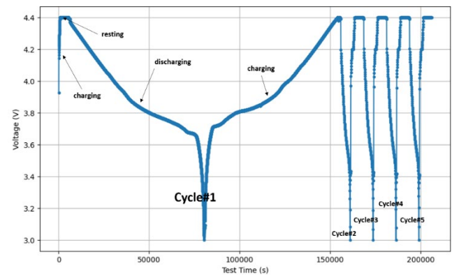
Figure 1. Voltage data for one sample of a pouch Li-ion battery
