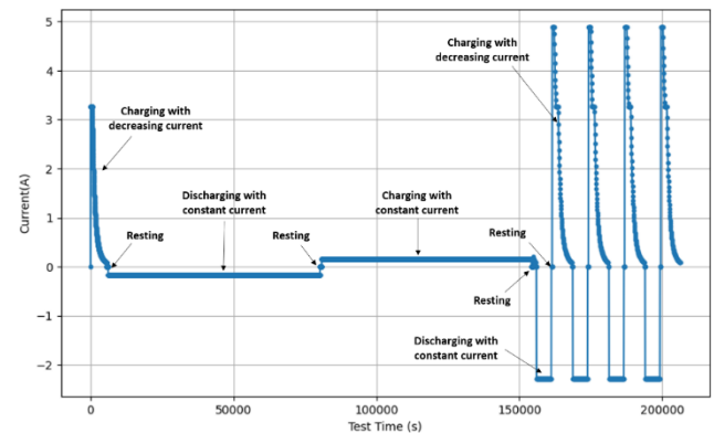
Figure 2. Current data for one sample of pouch Li-ion battery
