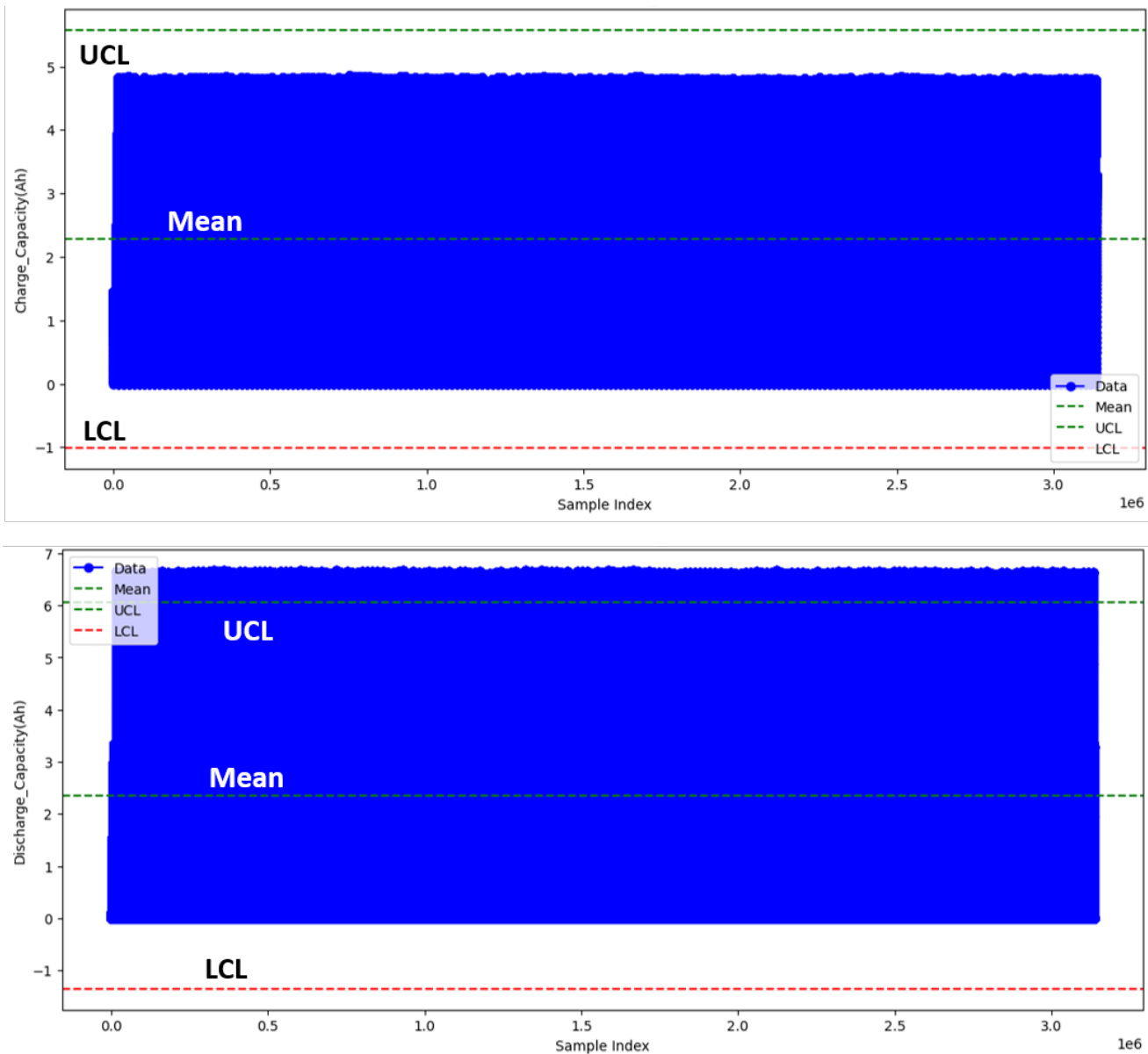
Figure 7. The control chart for charge and discharge capacities for all samples
