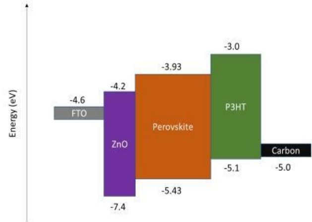
Figure 1. Energy band alignment of the device
