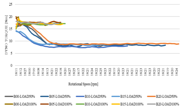
Figure 1. The torque changes from the dynamometer relative to the engine speed
