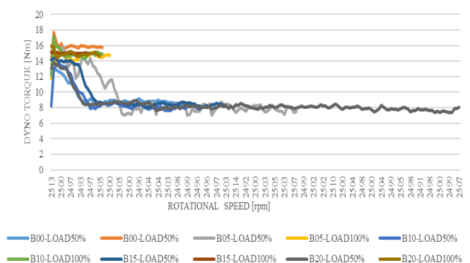
Figure 2. The torque changes from the dynamometer relative to the engine speed for the biodiesel blend
