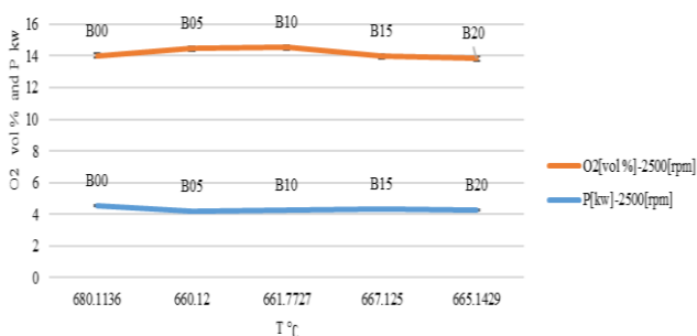
Figure 9. The rate of change in the percentage of oxygen and power in the engine load
