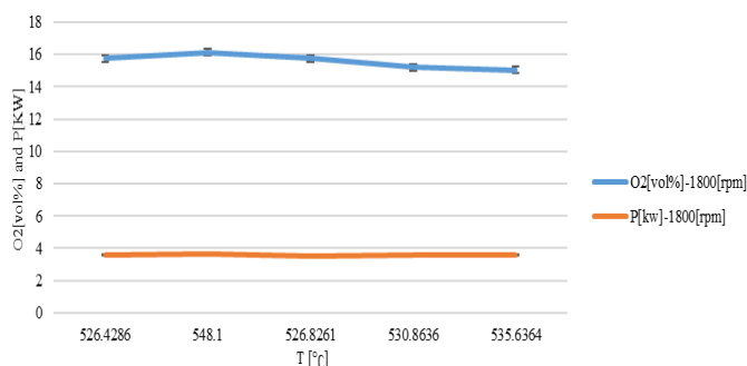
Figure 8. The rate of changes in the percentage of oxygen and power in the engine load
