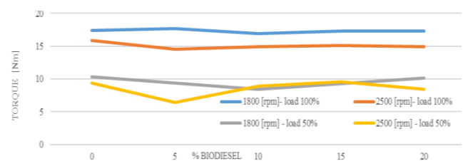
Figure 3. The Effect of adding biodiesel to diesel fuel on generating the engine's torque under test
