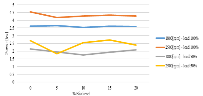
Figure 6. The Effect of biodiesel increases on the fuel blend on the brake power of the tested engine
