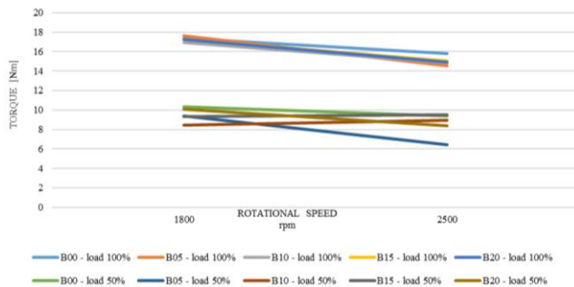
Figure 4. Effect of rotational speed on engine torque production under different biodiesel and diesel combinations
