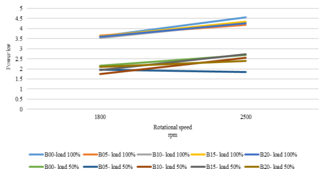
Figure 7. Effect of engine speed on the engine power
