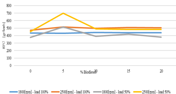
Figure 5. The effect of increasing the percentage of biodiesel composition in diesel fuel on fuel-specific consumption
