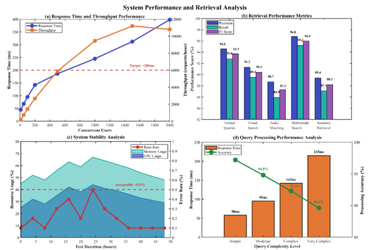
Figure 8. Comprehensive system performance and retrieval analysis of intelligent documentation platform (a) Response time and throughput performance under varying user loads, (b) Cross-modal retrieval performance evaluation across query types, (c) Long-term system stability and resource utilization analysis, (d) Query processing performance analysis by complexity level
