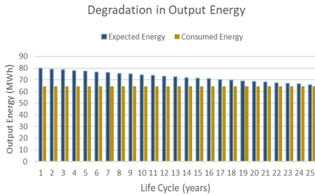
Figure 3. Degradation in the output energy during the life cycle
