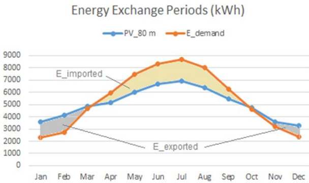
Figure 8. Periods of energy exchange in case of using 80 modules PV array
